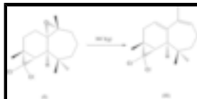
Fig. 2. The formation of the title compound.
